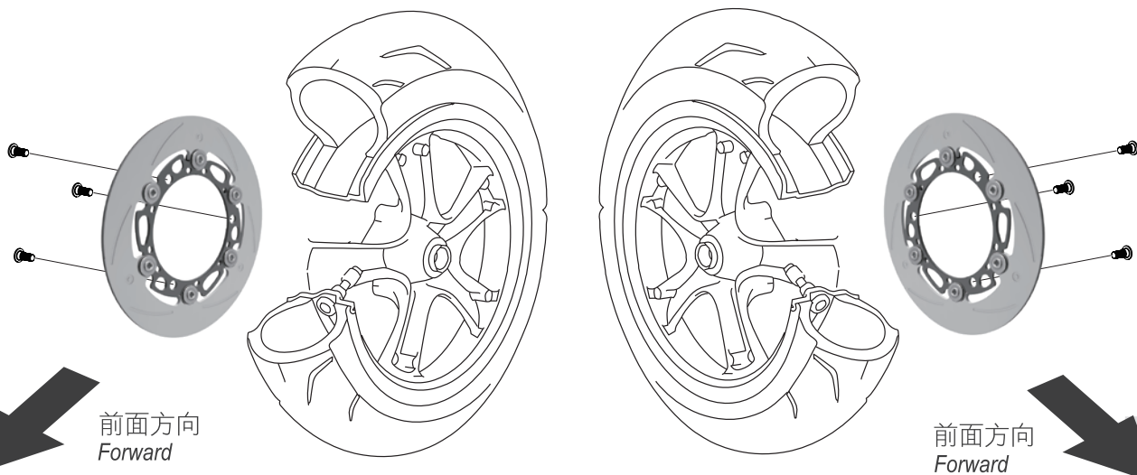
Right front brake disk
