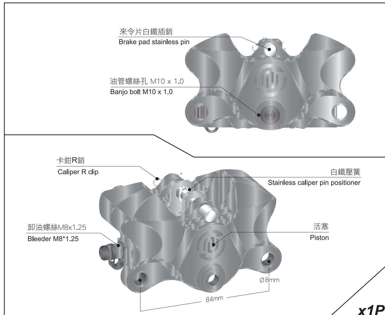
螃蟹對二卡鉗 / CNC 2 POT CRAB CALIPER
