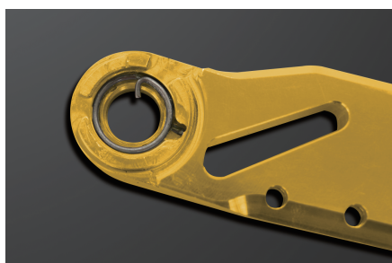
6.將旋轉彈簧置入NCY之腳踏桿內部，旋轉彈簧置入時方向要與原廠相同。 Install the rotating spring into NCY footrest rod, direction of rotating spring must be same with original one.
